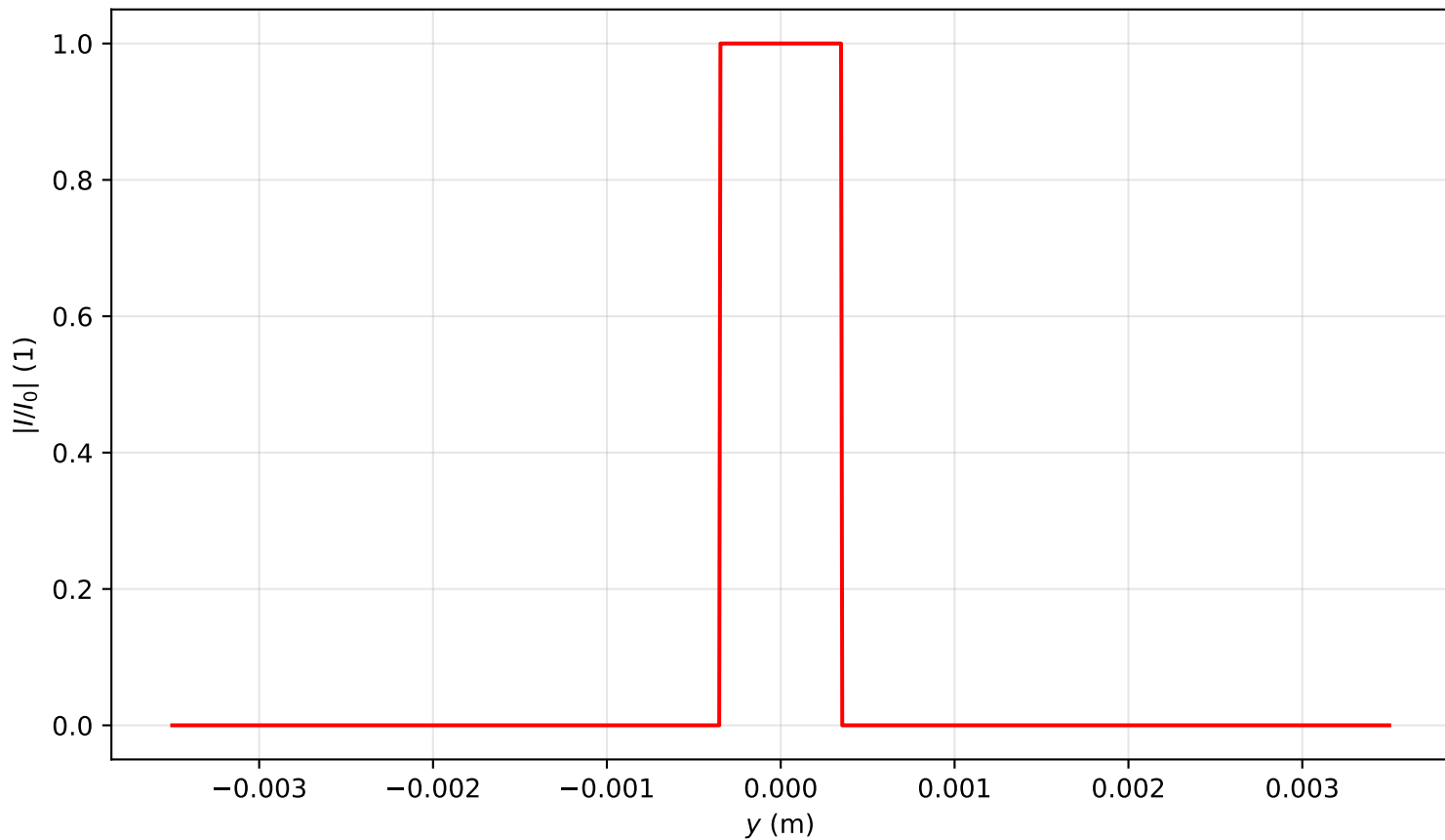
Intensity profile I(x = 0, y, z = 0.000)/I_0 , P_{in}=2.0P_{cr} , artificial time
